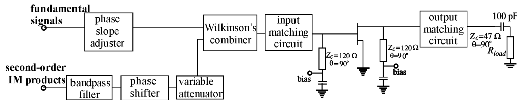
Fig. 1. Amplifier with injection of the second harmonics
